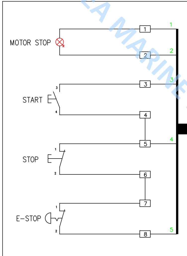
TYPICAL WIRING DIAGRAM INSIDE JB
